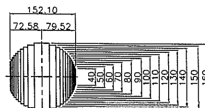
CORE CROSS SECTION AREA OF CORE 192.65 cm 2
