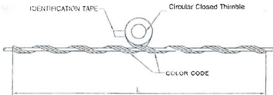
Figure 1 The Thimble preformed suspension for the cable.
