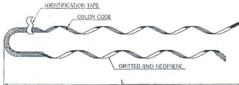
Figure 1 Preformed dead-end
