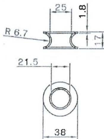
Figure 1 The Thimble preformed suspension for the cable.
