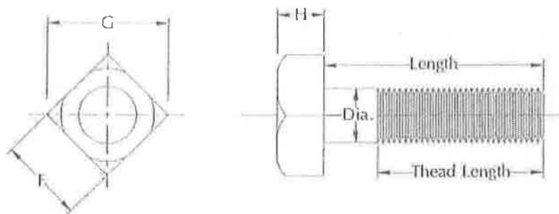
Figure 1 Machine Bolt Head
