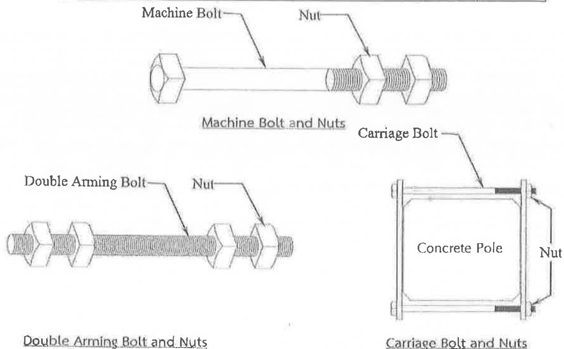
Figure 2 Machine Bolt, Double Arming Bolt and Carriage Bolt
