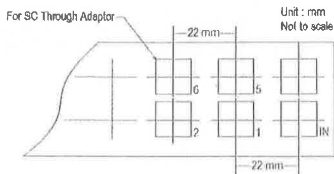
Figure 2 The panel of Splitter Box
