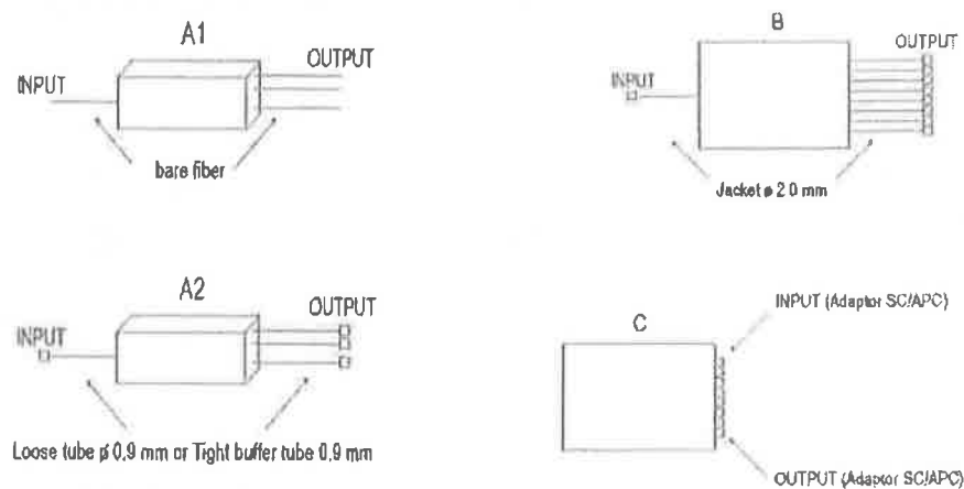
Figure 1 Type of splitter
