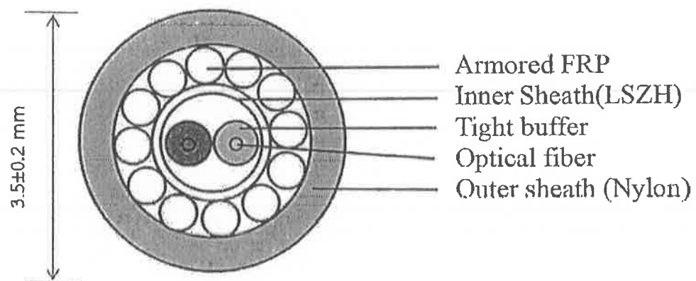
Figure 2 Cross section of 2 fibers cable
