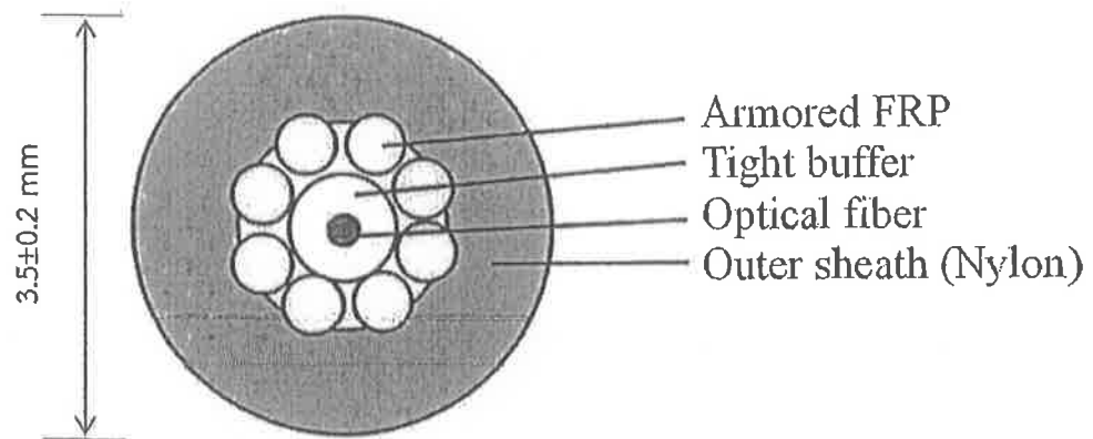
Figure 1 Cross section of 1 fiber cable
