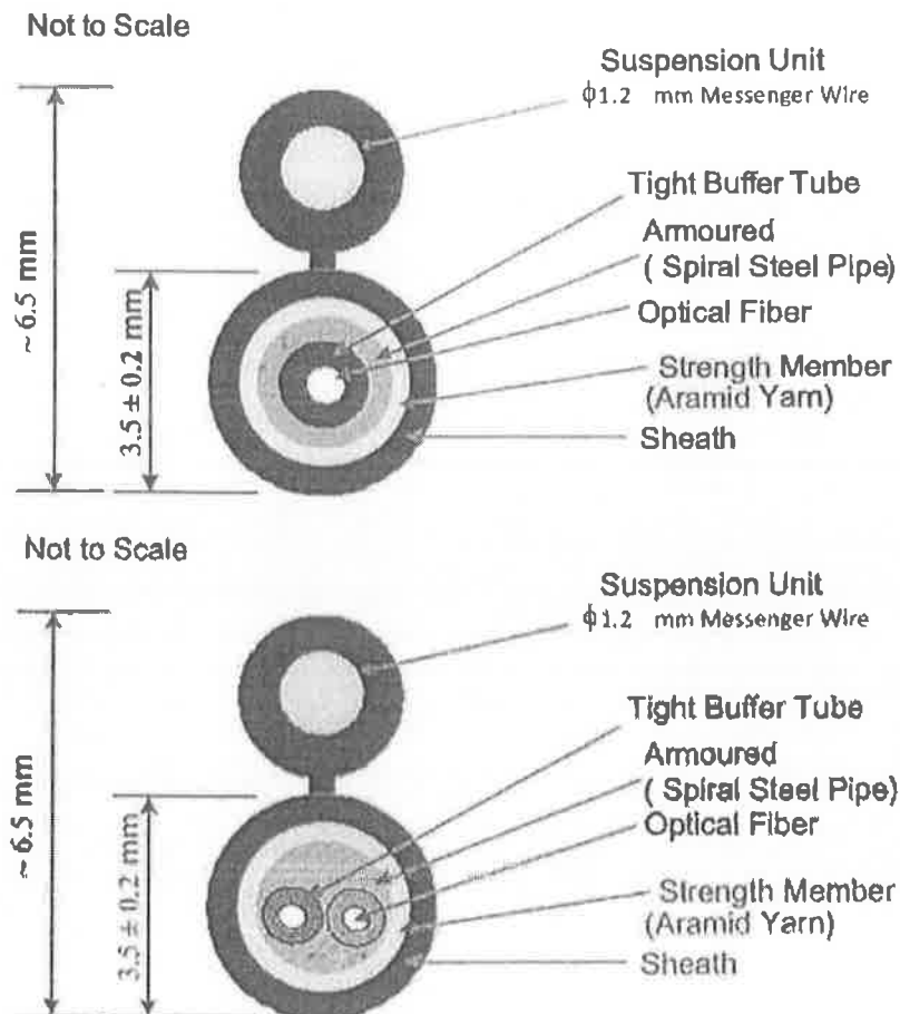
Figure 1 Cross section of 1 and 2 fibers cable
