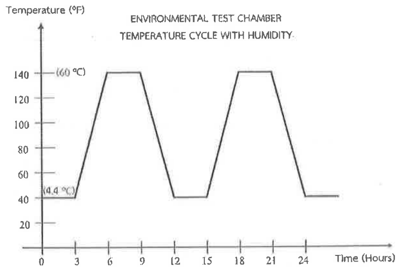
Figure 8 Temperature Cycling
