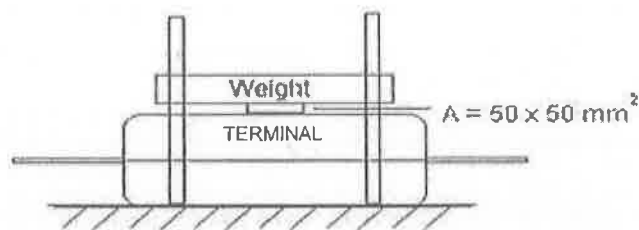
Figure 4 Compression
