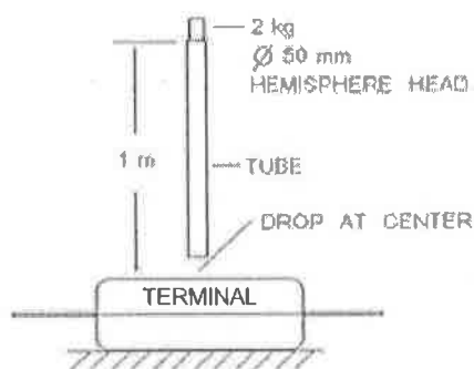
Figure 5 Impact
