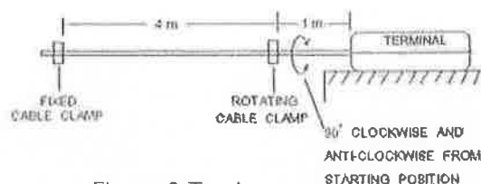
Figure 3 Torsion
