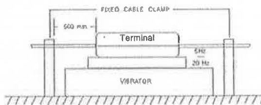
Figure 6 Vibration
