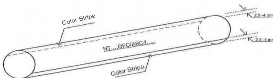
Figure 2 Cable Making
