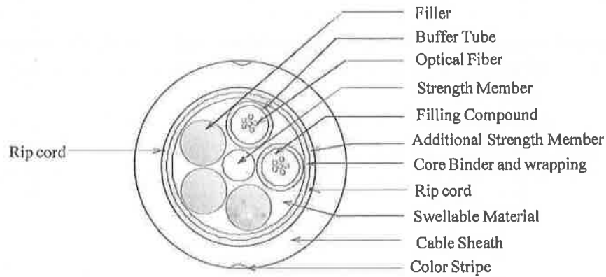
Figure 1 Cross-Section of ADSS OFC 12 fibers
