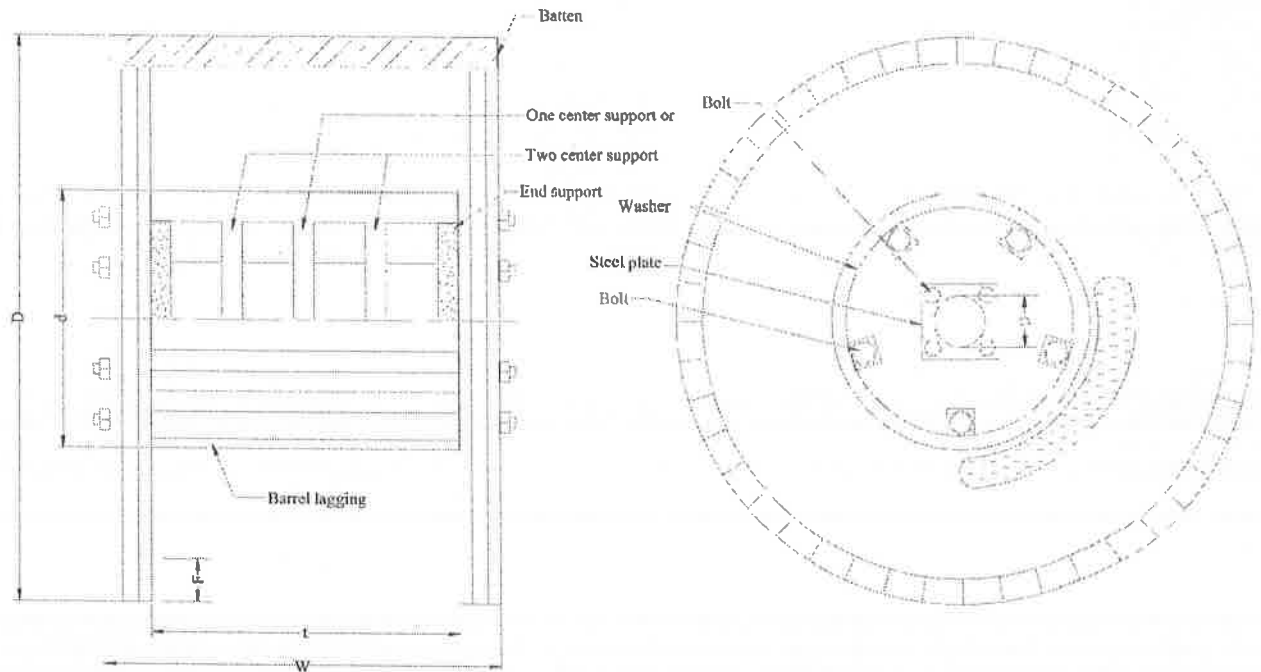
Figure I. wooden cable drum
