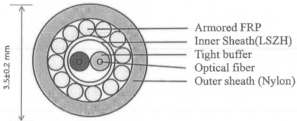
Figure 2 Cross section of 2 fibers cable
