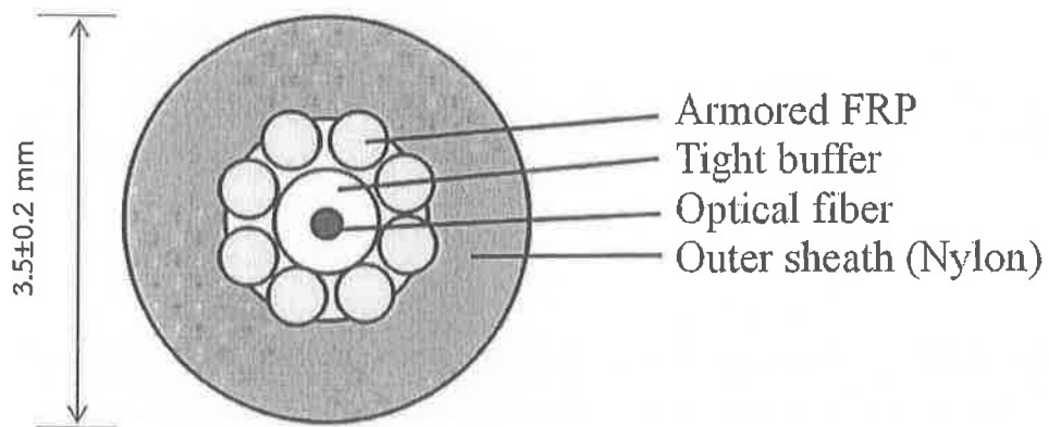
Figure 1 Cross section of 1 fiber cable
