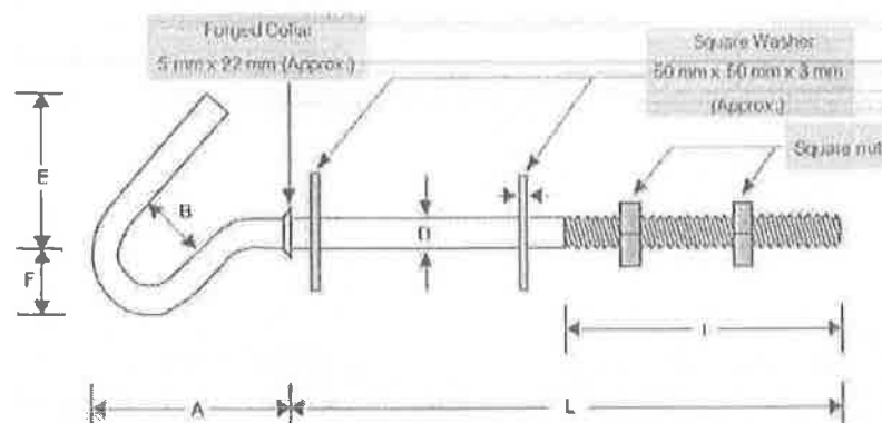
Figure 1 Hook Bolt
