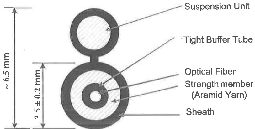
Figure 1 Cross section of 1 fiber cable
