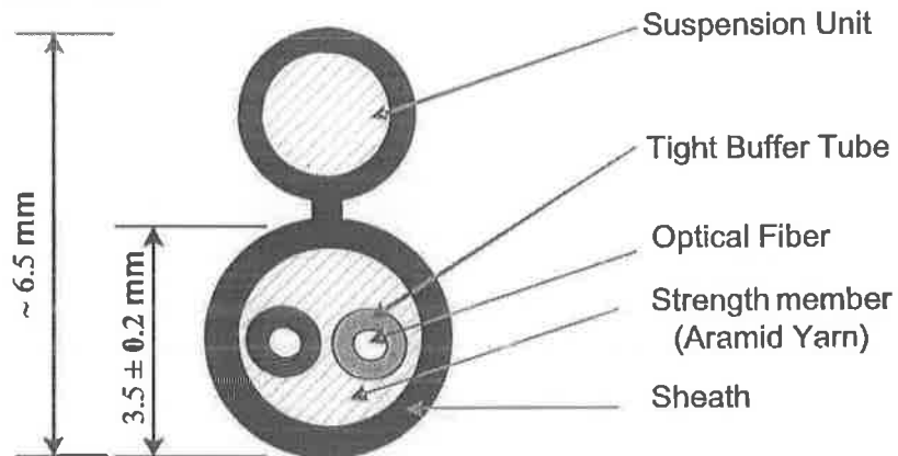
Figure 2 Cross section of 2 fiber cable
