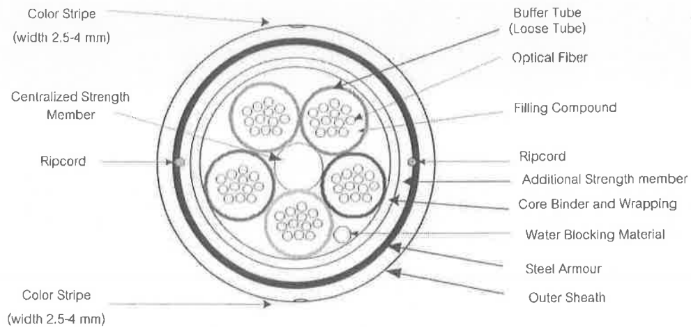
Figure 3 ARSS OFC 60 Core
