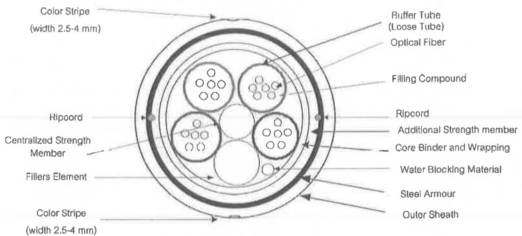
Figure 2 ARSS OFC 24 Core
