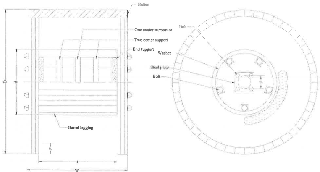
Figure I. wooden cable drum
