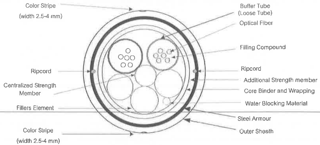
Figure 1 ARSS OFC 12 Core
