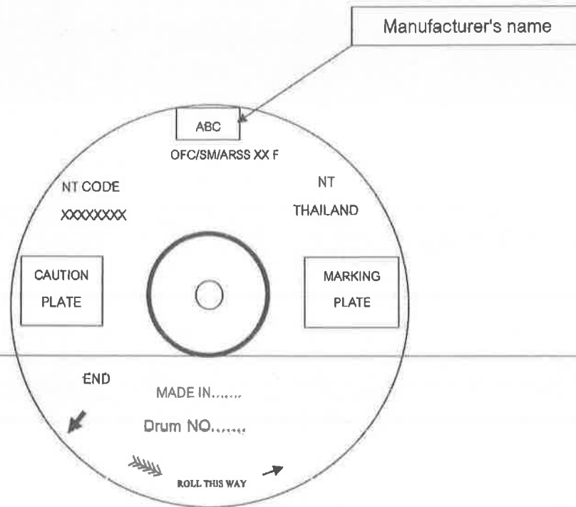
Figure 5 Cable-drum marking
