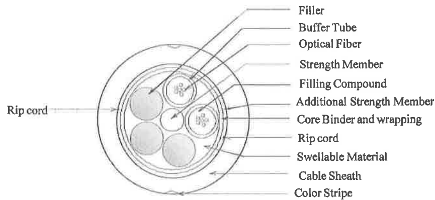
Figure 1 Cross-Section of ADSS OFC
