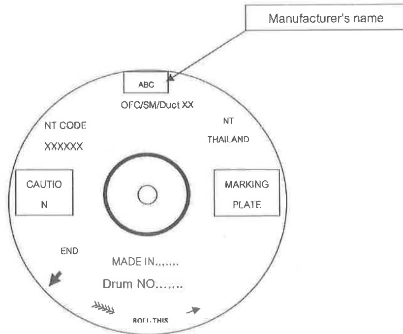
Figure 5 Cable-drum marking
