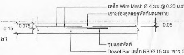
CONTRACTION JOINT
