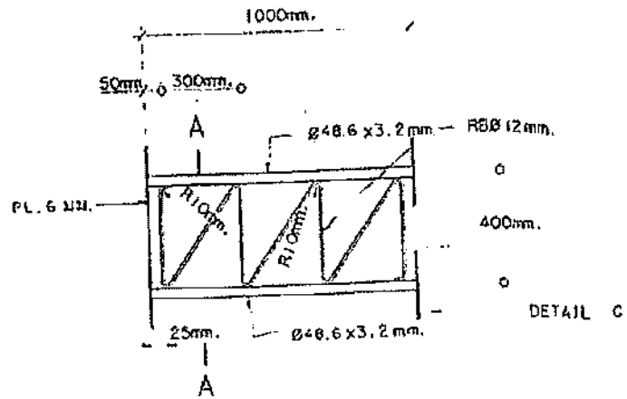
TOWER 1 1:20
