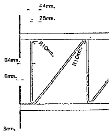
DETAIL C 1:10
