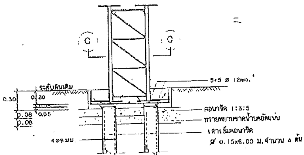
TOWER 1 1:20
