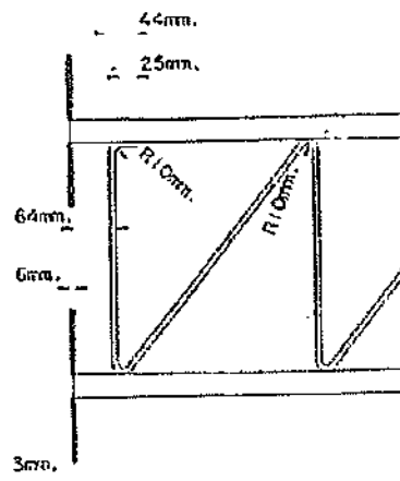
DETAIL C 1:10
