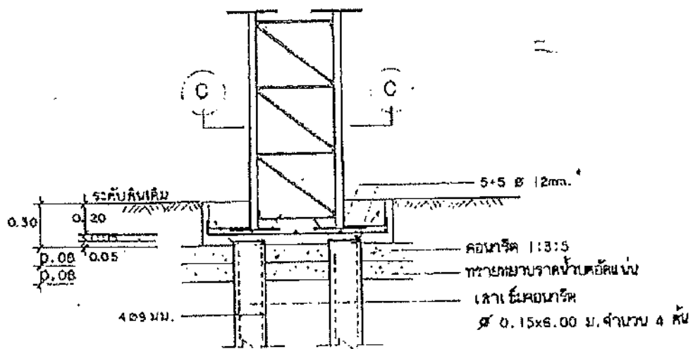
TOWER 1 1:20
