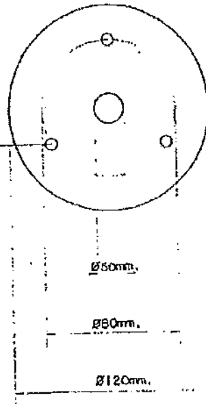
DETAIL B 1:5
