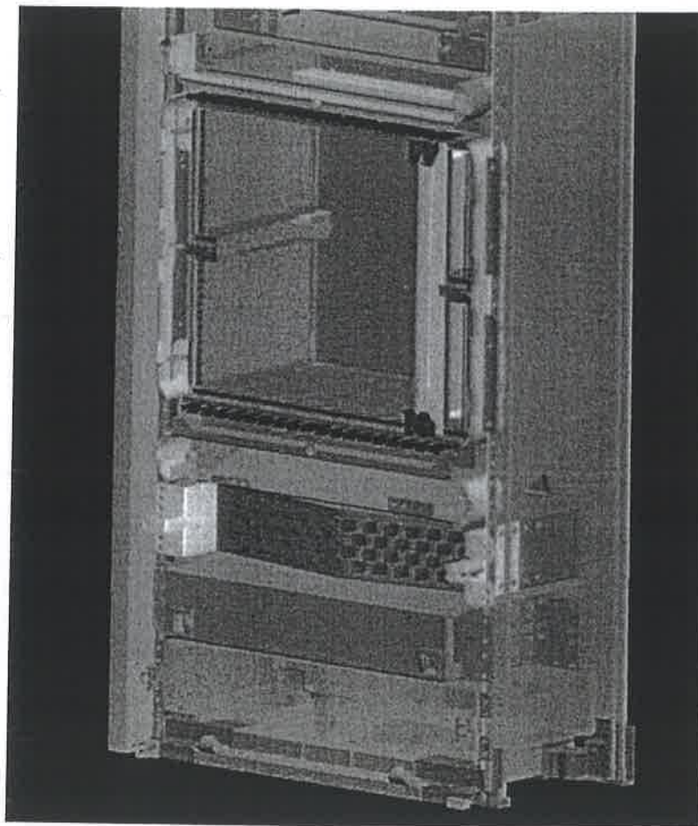
Figure 5-93 Subrack mounted in an ETSI rack
