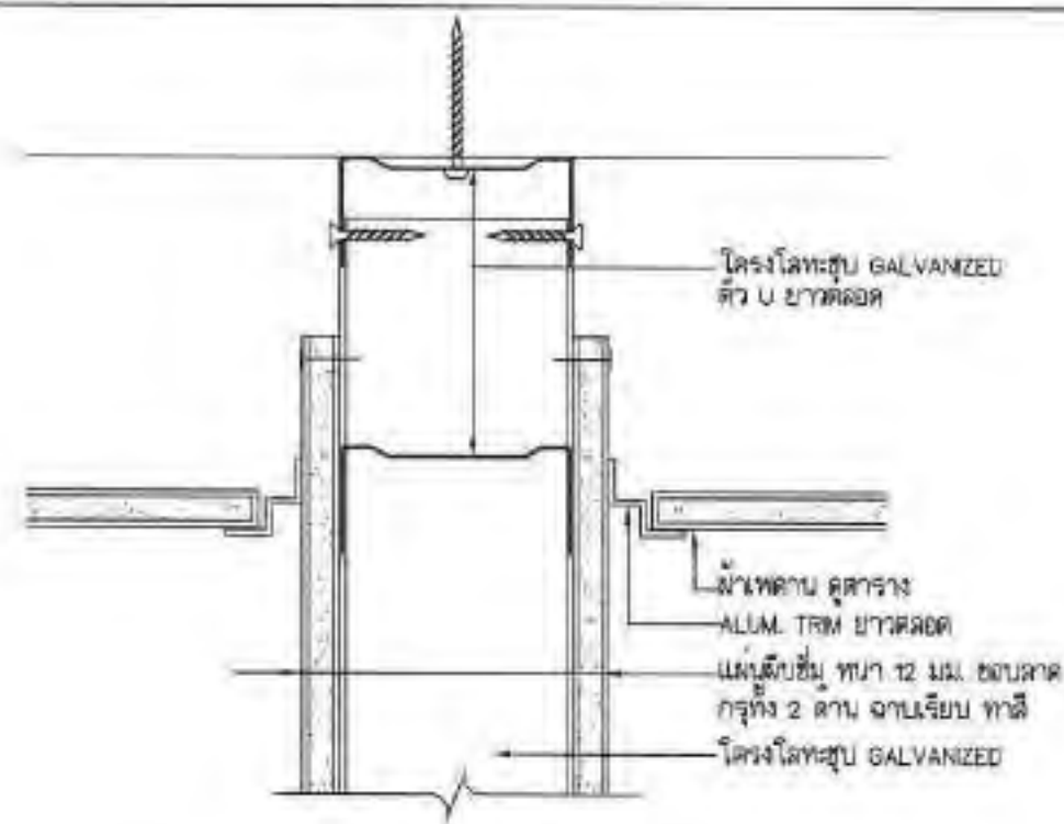
CEILING (t-bar) SECTION SCALE 1:2.5
