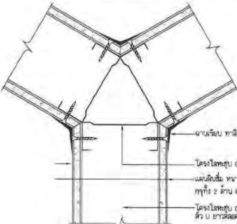
"Y" CORNER PLAN SCALE 1/25
