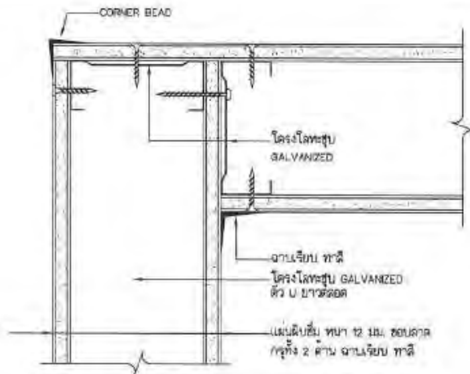
"T" CORNER PLAN "90" CORNER PLAN SCALE 1/25 SCALE 1/25
