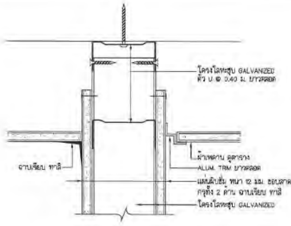
CEILING (plaster) SECTION SCALE 1/25
