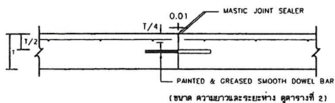
CONSTRUCTION JOINT
