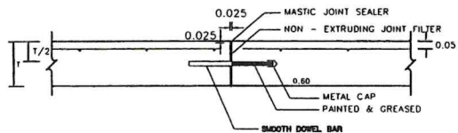
EXPANSION JOINT
