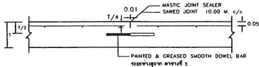
CONTRACTION JOINT
