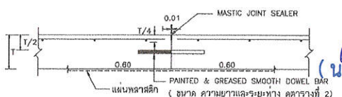
CONSTRUCTION JOINT
