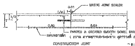
CONSTRUCTION JOINT
