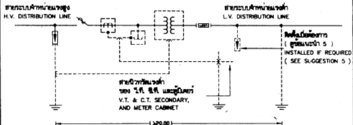
EARTHING DIAGRAM
