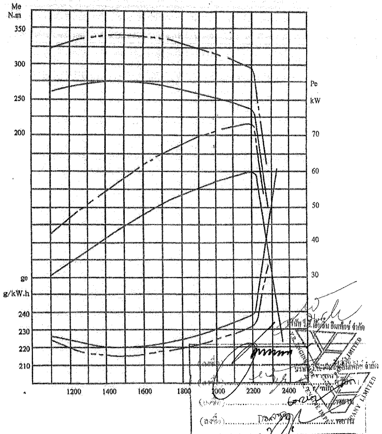
Fig. 3 Speed and speed adujsted characteristic curve for Model R4105, R4105Zd diesel engine
